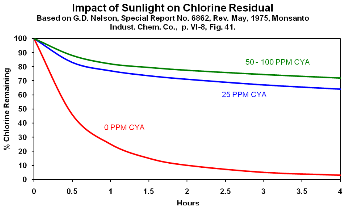
Figure 1. Impact of sunlight on chlorine residual
